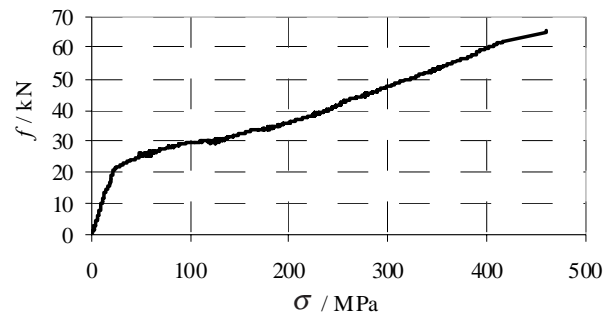
Fig. 23 Increase of stress in tensile reinforcing bar with applied load
