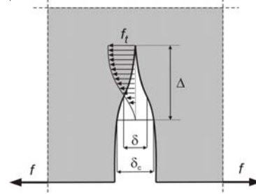
Fig. 2 Single crack model for the softening part of the stress-strain diagram
