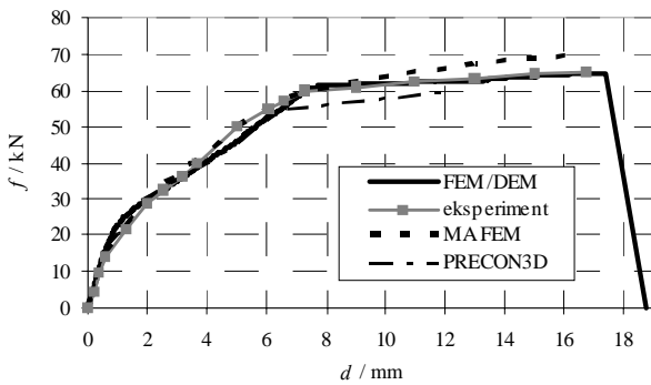
Fig. 22 Load-displacement curves for the mid-span of the beam
