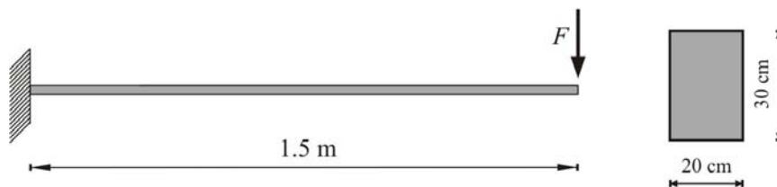
Fig. 13 Geometry and load of structure
