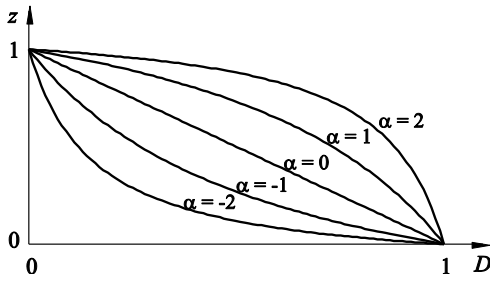
Fig. 8 Reduction factor for different values of shape parameter \alpha
