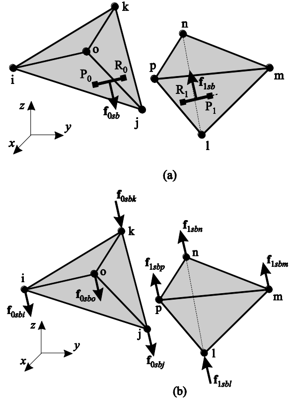
Fig. 13 Steel bolt: (a) force in steel bolt; (b) equivalent nodal forces
