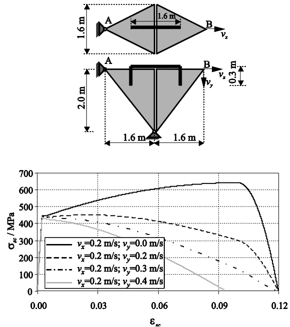
Fig. 10 Stress-strain relation in steel clamps for different cases of loading
