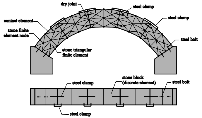
Fig. 3 Discretization of dry stone structure with steel clamps and bolts.
