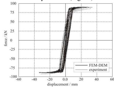
Fig. 18 Force-displacement diagrams under cyclic loading
