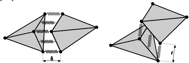
Fig. 5 Normal and shear springs between the finite elements
