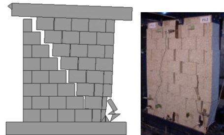
Fig. 19 Failure patterns of dry masonry wall (numerical and experimental)
