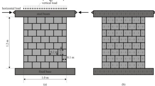
Fig. 15 Dry stone masonry wall: (a) geometry; (b) finite element mesh
