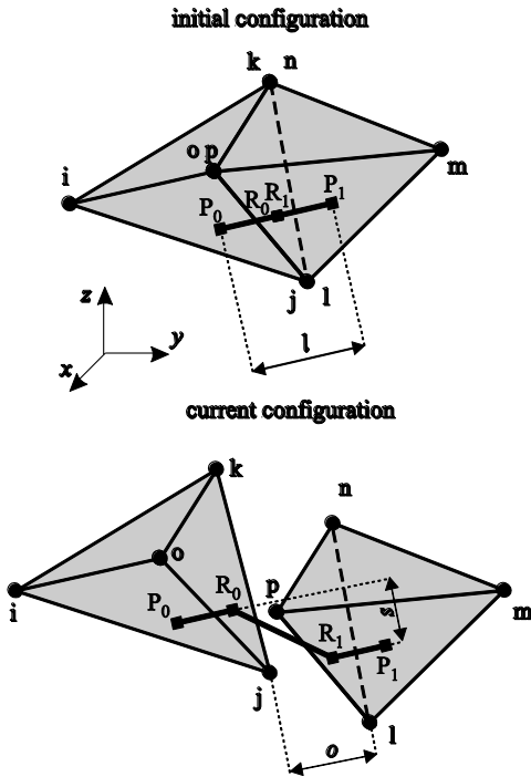
Fig. 11 Steel bolt in initial and current configuration
