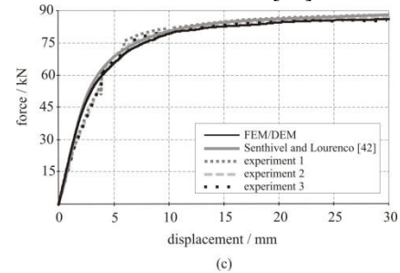
Fig. 17 Force-displacement diagrams under monotonic loading
