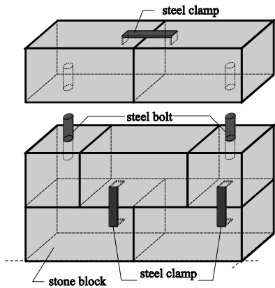
Fig. 2 Steel clamps and bolts
