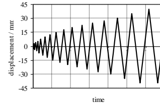
Fig. 16 Loading history
