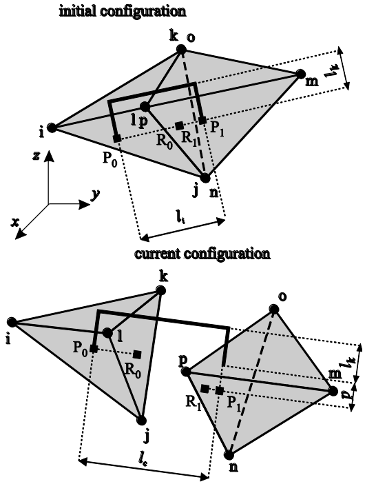
Fig. 7 Steel clamp in initial and current configuration.
