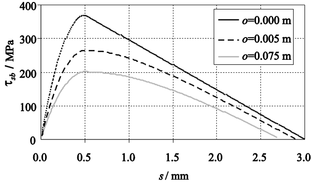
Fig. 14 Shear stress - shear separation relations in steel bolt for different initial normal separation \sigma
