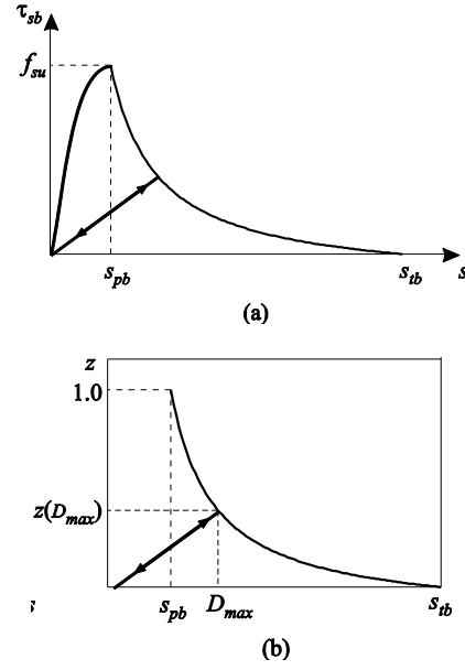
Fig. 12 Material model in the steel bolt: (a) shear stresses versus shear separation, (b) cyclic behavior
