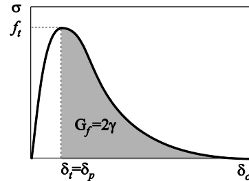
Fig. 4 Strain softening stress-strain and stress-displacement curves
