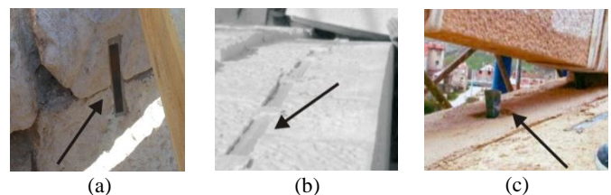
Fig. 1 Steel clamps and bolts: (a) steel clamp embedded on the lateral face of the structure; (b) steel clamp embedded on the top side of stone blocks; (c) steel bolts [17].
