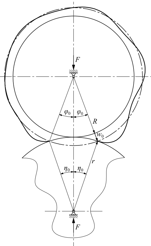
Fig. 7 Tyre standing waves, \Omega = 230 \text{ rad/s} , V = 248 \text{ km/h}
