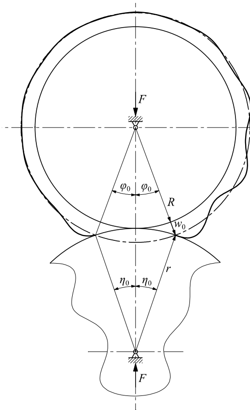
Fig. 6 Tyre standing waves, \Omega_2 = 215.38 \text{ rad/s} , V = 233 \text{ km/h}
